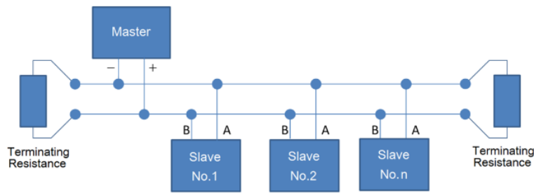
Figure 5-4-3. Connections of C-BOX in a Modbus 485 network
