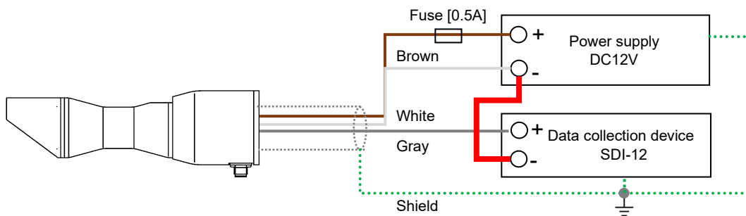
Figure 5-7. How to connect MS-57SH (SDI-12)
