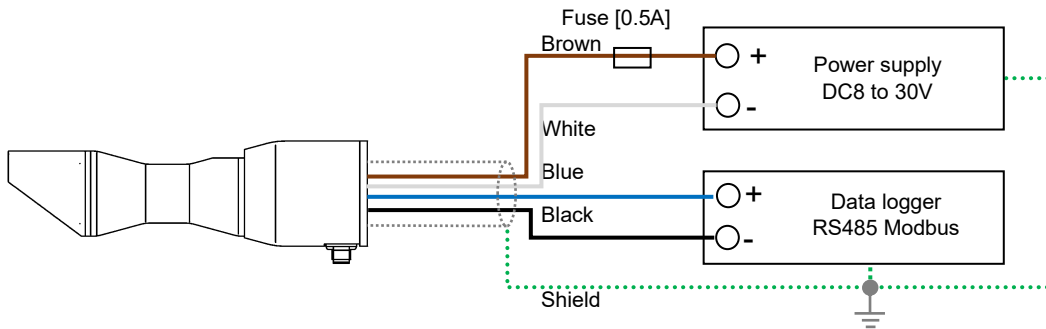
Figure 5-5. How to connect MS-57SH (Modbus RTU RS485)
