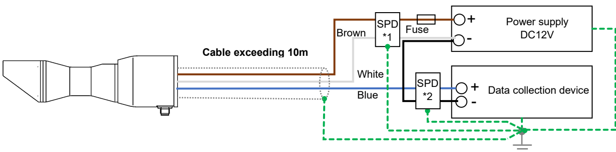
Figure A9-2. SDI-12 connection (when the cable length exceeds 10m, etc.)
