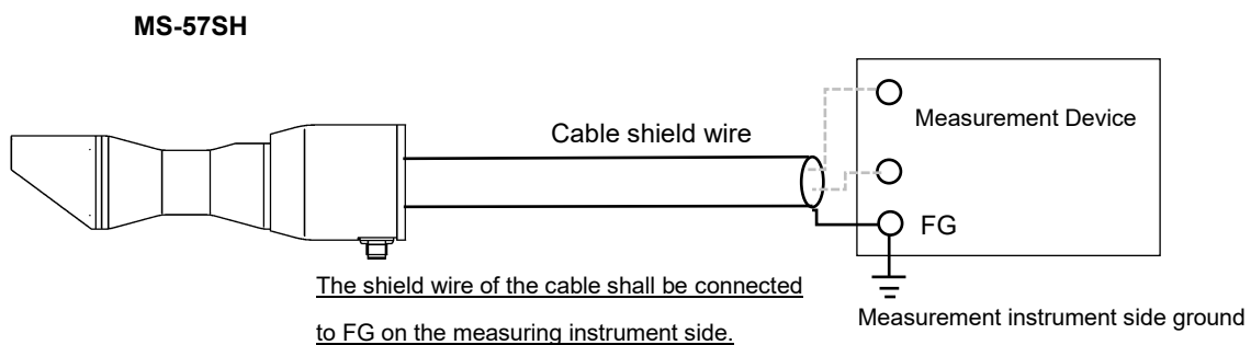
Figure 5-3. MS-57SH ground connection method
