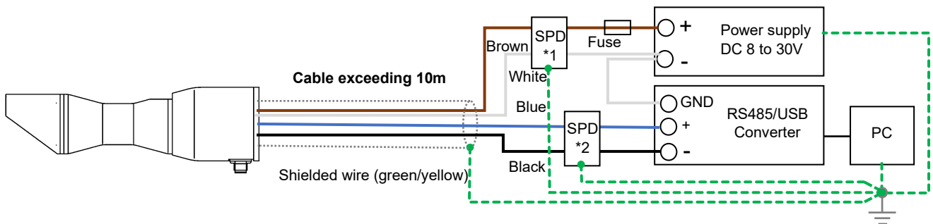
Figure A9-1. Modbus RTU connection (when the cable length exceeds 10m, etc.)
