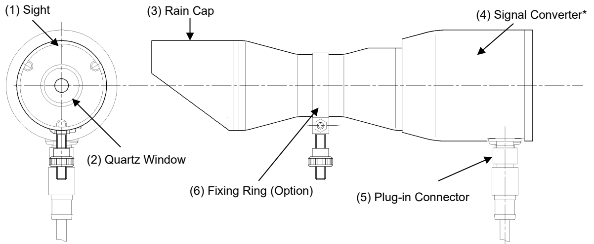
Figure 5-1. Pyrheliometer Parts Name [MS-57SH]
