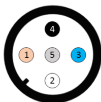
Figure 5-9. Connector pin number of the MS-57SH
