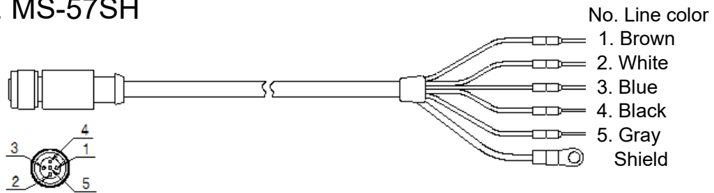
Figure 7-2. Output Cables
