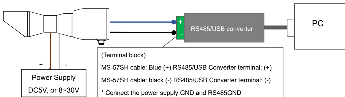
Figure A3-1. Hardware preparation
